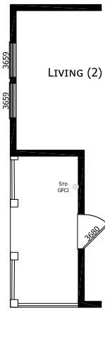
OPTIONAL RECESSED PORCH (add 6' to LR)
